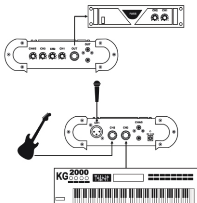
Connection example
